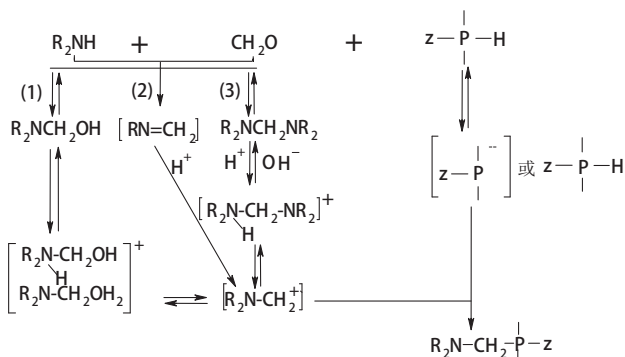
Figure1 Schematic Figure of Die Mannich Reaction
